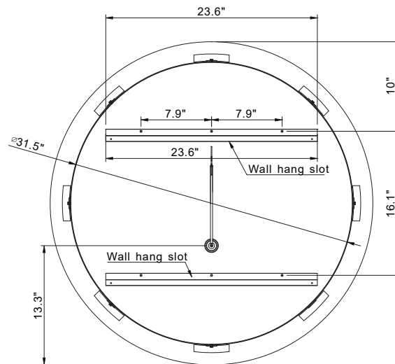
REAR VIEW
