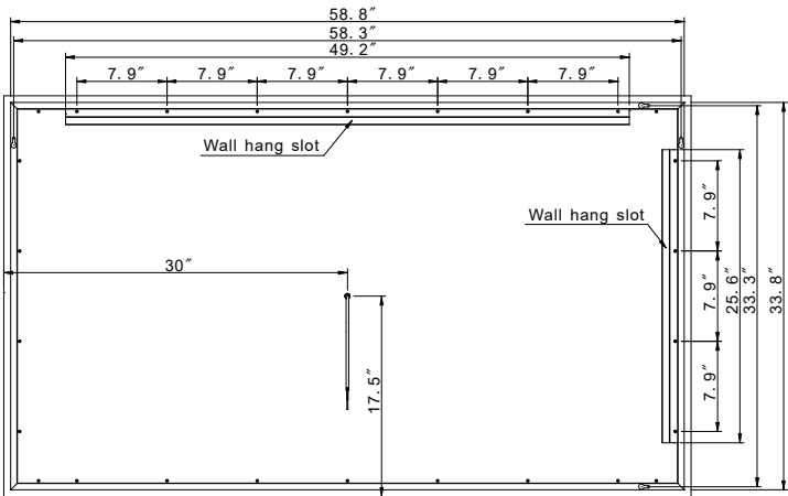
REAR VIEW
