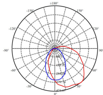
7W Light Distribution Curve →
