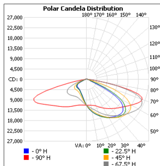
Knuckle LCFLD-BRACKET-K
