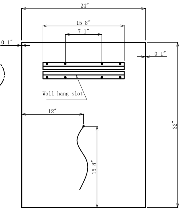
REAR VIEW
