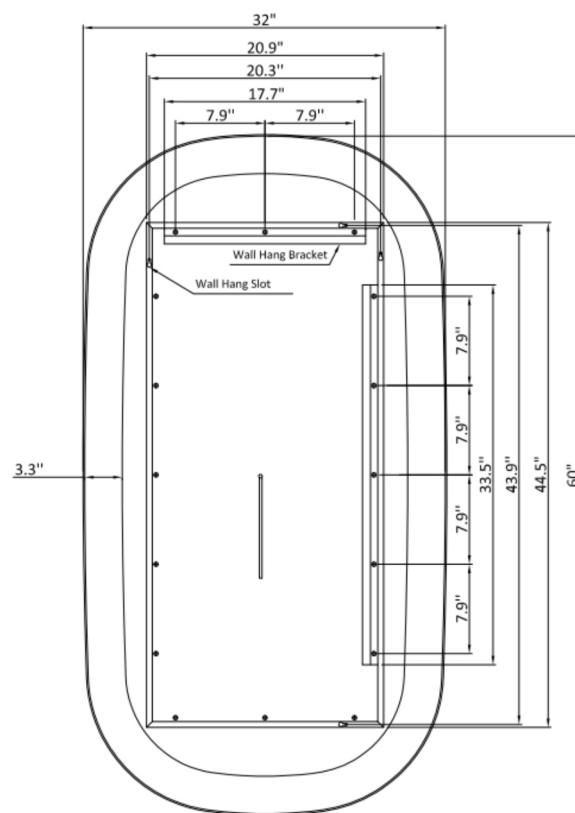
REAR VIEW
