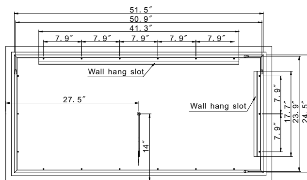
REAR VIEW
