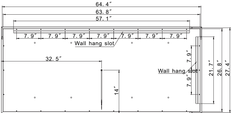
REAR VIEW
