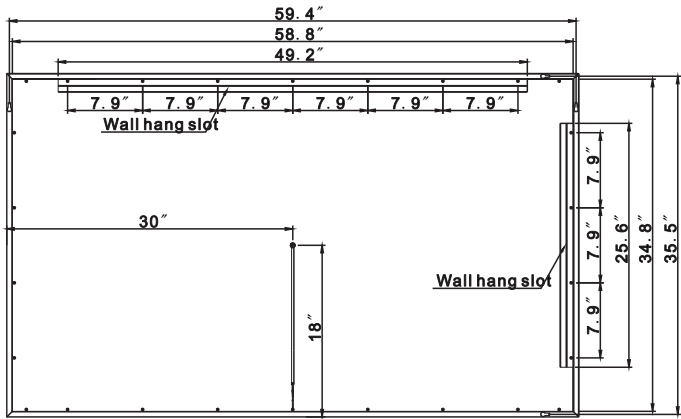
REAR VIEW
