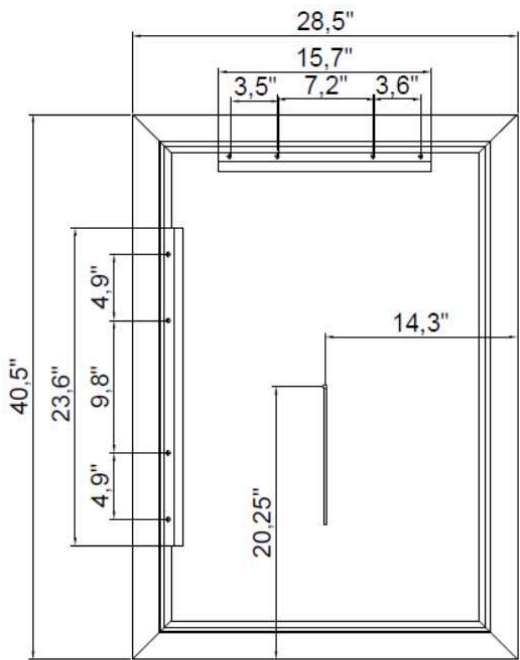
REAR VIEW
