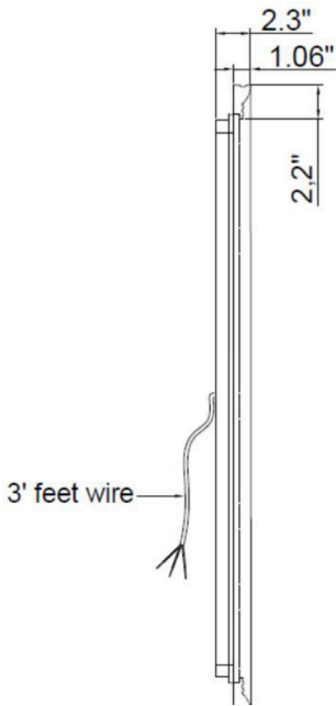
LEFT VIEW
