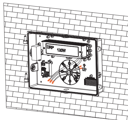
Step 6: Wiring
