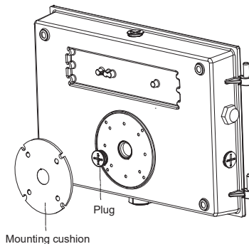
Step 4: Punch the hole plug and stick the installation buffer pad behind the bottom cover
