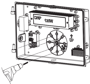
Step 3: Drill holes in the bottom cover and select the hole location to be installed according to the actual situation
