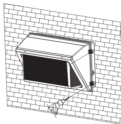
Step 8: Fix the lamp body to the bottom cover and apply glue around the lamp body
